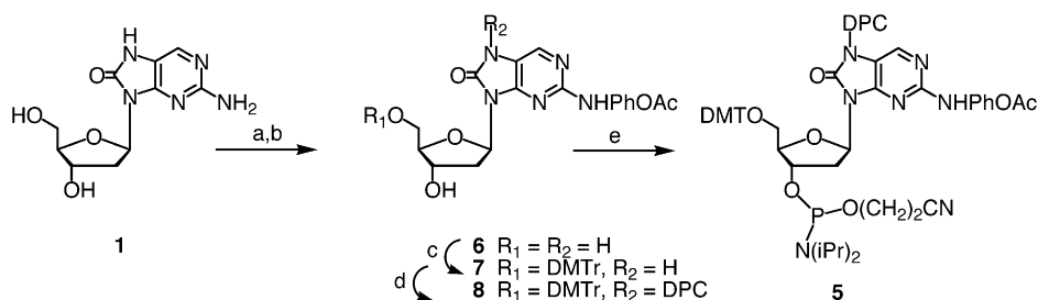
Scheme 2. Reagents and conditions: (a) phenoxyacetyl chloride, pyridine, 30 min; (b) 0.5 N sodium methylate, 30 min, 62%; (c) DMTCl chloride, pyridine, 2 h, 76%; (d) diphenylcarbamoyl chloride, DIPEA, pyridine, 2 h, 61%; (e) 2-cyanoethyl- N,N -di- iso -propylchlorophosphoramidite, DIPEA, CH 2 Cl 2 , 30 min, 77%.
