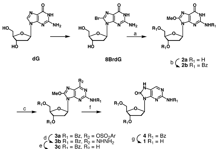
Scheme 1. Reagents and conditions: (a) 3 N sodium methylate, reflux, 72 h, 77%; (b) benzoyl chloride, pyridine, 1 h, 62%; (c) 2,4,6-tri- iso -propylbenzenesulfonyl chloride, DIPEA, CH 2 Cl 2 , 1.5 h, 64%; (d) anhydrous hydrazine, THF, 6 h; (e) Ag 2 O, THF-5% H 2 O, reflux, 2 h, 38%; (f) thiophenol, triethylamine, DMF, 60 °C, 2.5 h, 80%; (g) 2N NaOH, pyridine/methanol; then 33% aqueous ammonia, 55 °C, 48 h, 63%.
