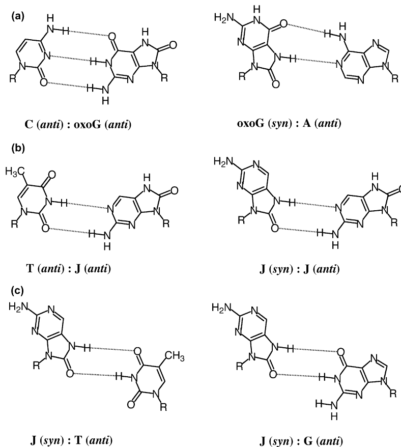
Figure 1. Proposed structures of hydrogen-bonded base pairs involving 2-amino-8-oxopurine (J) compared to those of 8-oxoguanine (oxoG).
